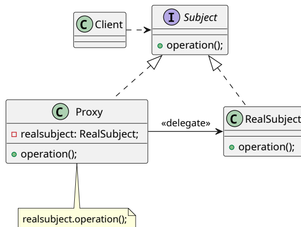
Figure 317: Diagram of the Proxy Pattern
